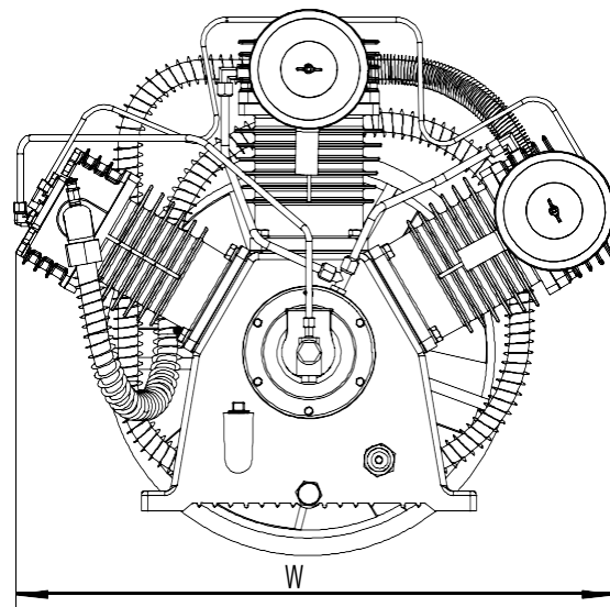
MODEL C3 TWO STAGE AIR COMPRESSOR PUMP
