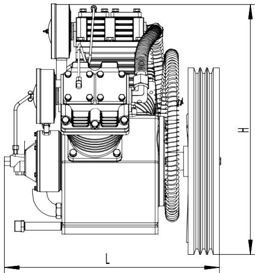
MODEL C3 TWO STAGE AIR COMPRESSOR PUMP
